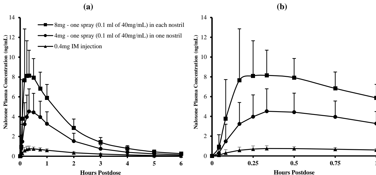
Figure 1 Mean ± SD Plasma Concentration of Naloxone, (a) 0-6 h and (b) 0-1h Following Intranasal Administration and Intramuscular Injection
