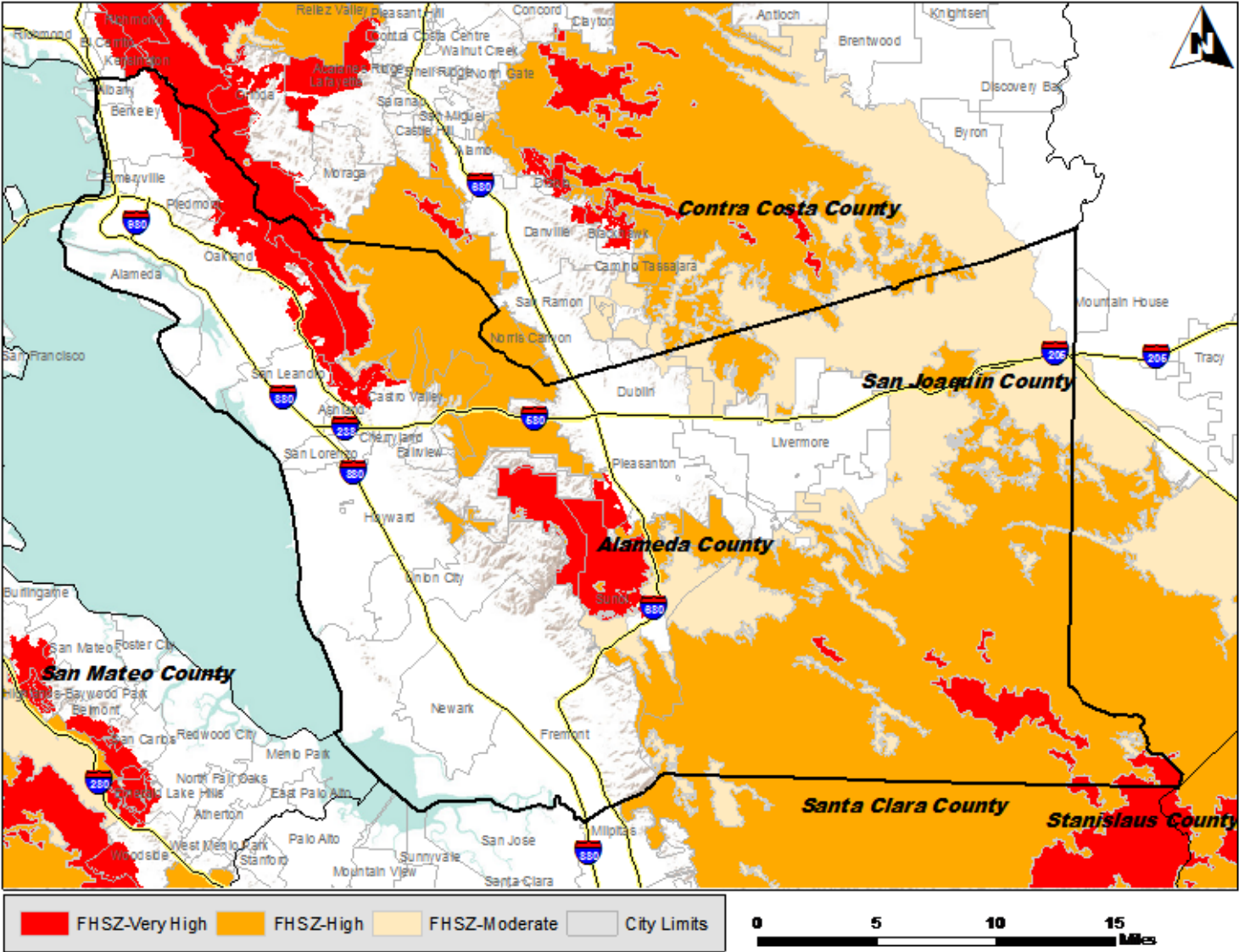
Figure 3. Current Fire Hazard Severity Zones (FHSZ), Alameda County, 2007. 9
