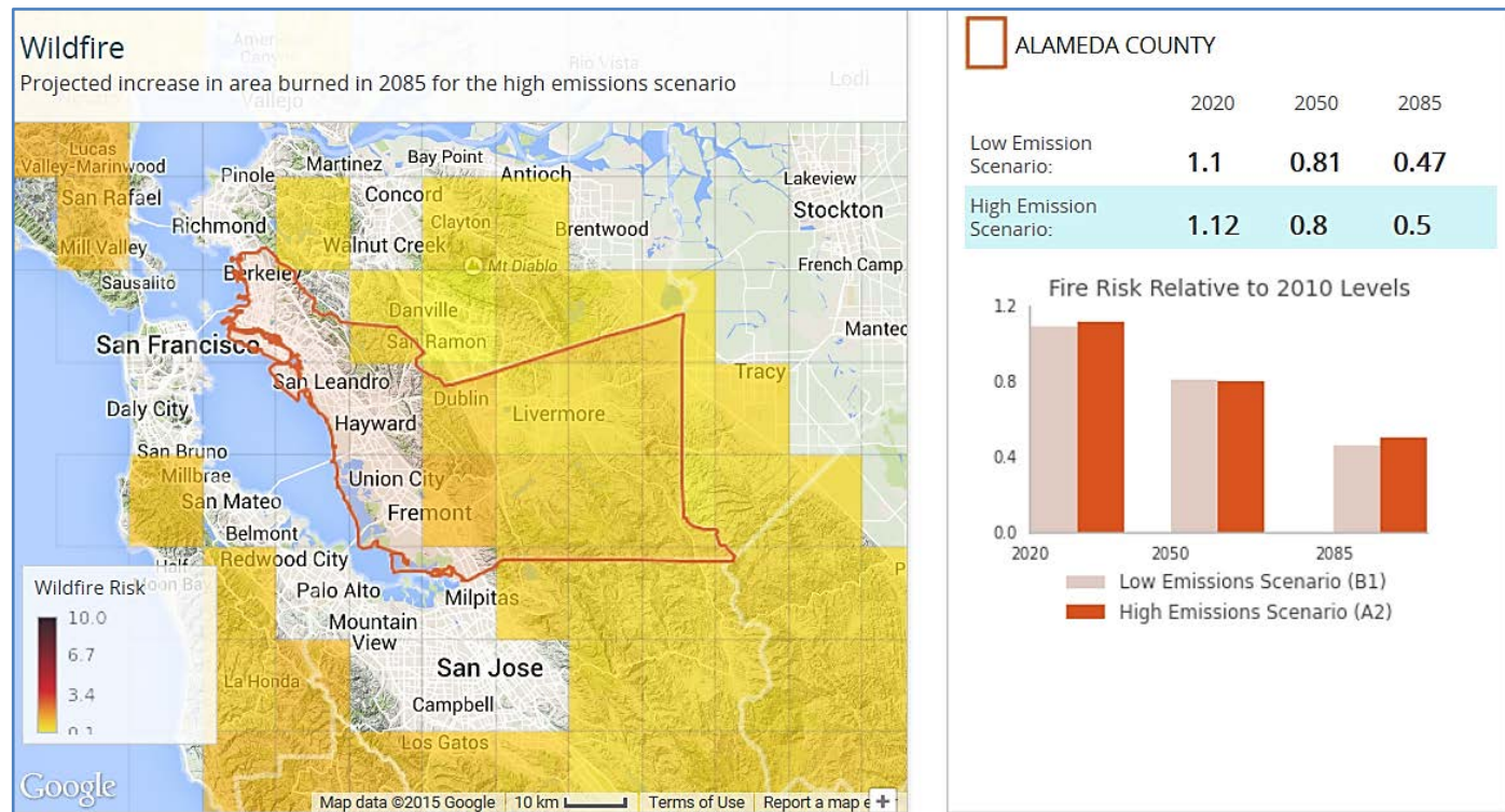
Figure 4. Relative increase in wildfire acreage in future carbon emission scenarios, Alameda County 6
