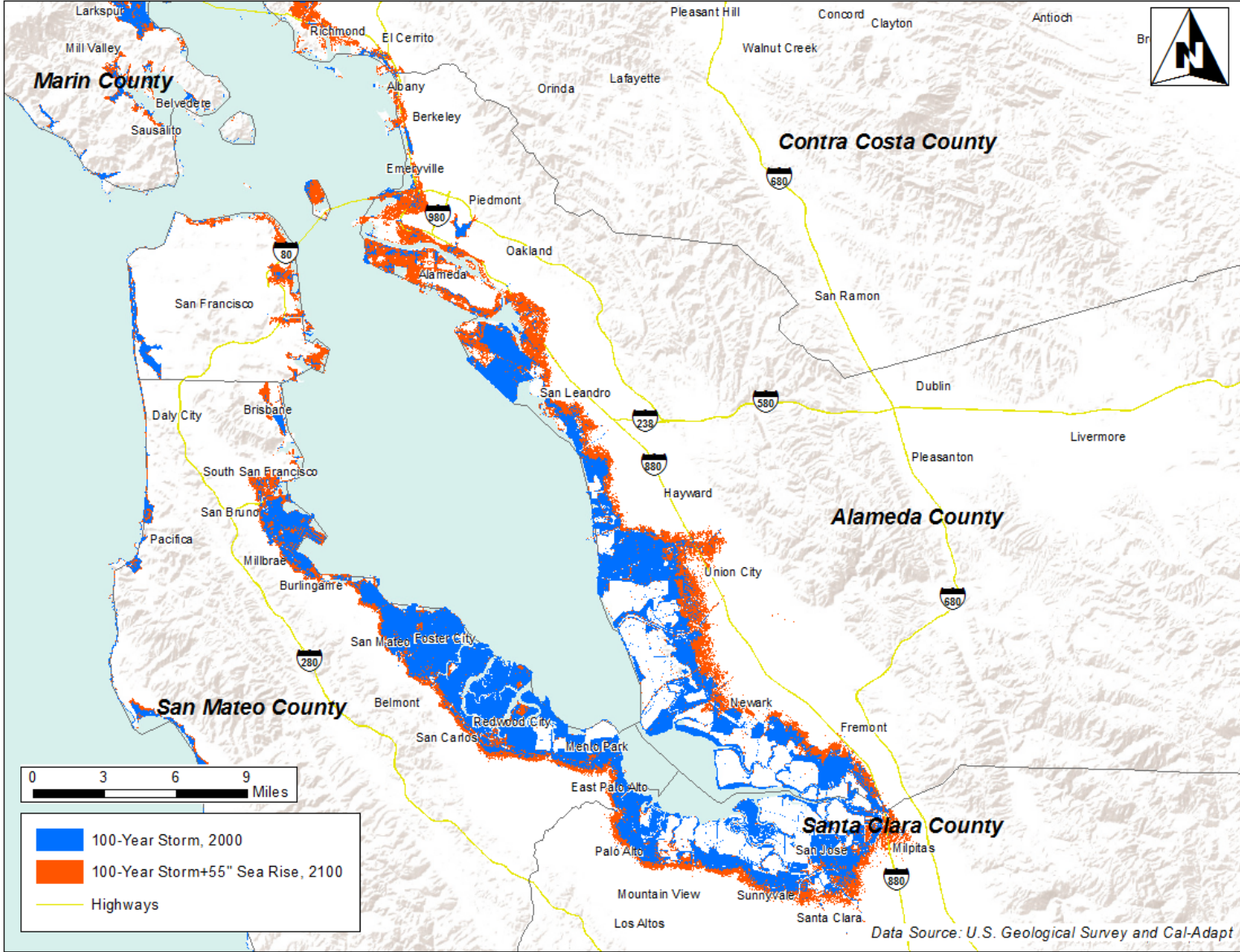
Figure 5. Baseline inundation areas for a 100-year flood (2000) and modeled scenario with additional 55 inches of sea level rise (2100), Alameda County 6 Note: Current SLR projections are 66 inches above sea level. 7
