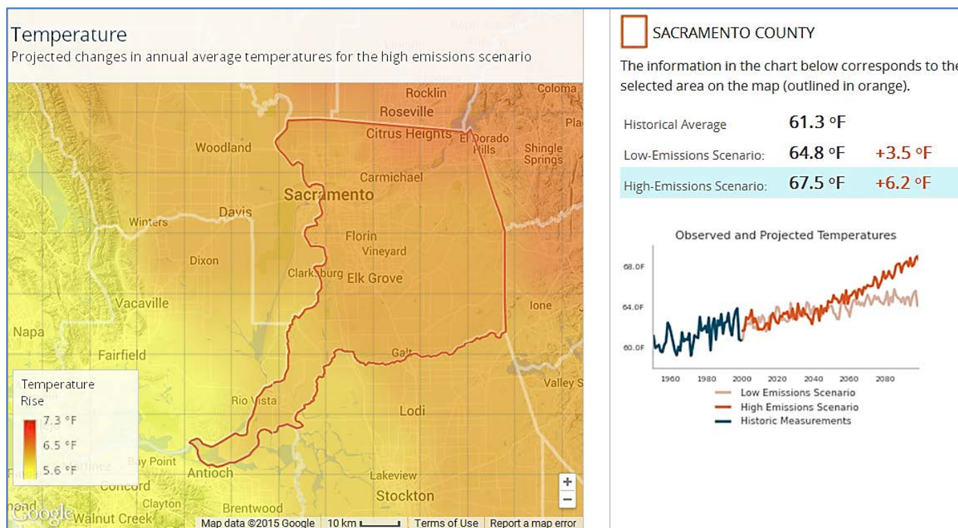
Figure 2. Projected changes in annual average temperature in future carbon emissions scenarios, Sacramento County, 2099 6
